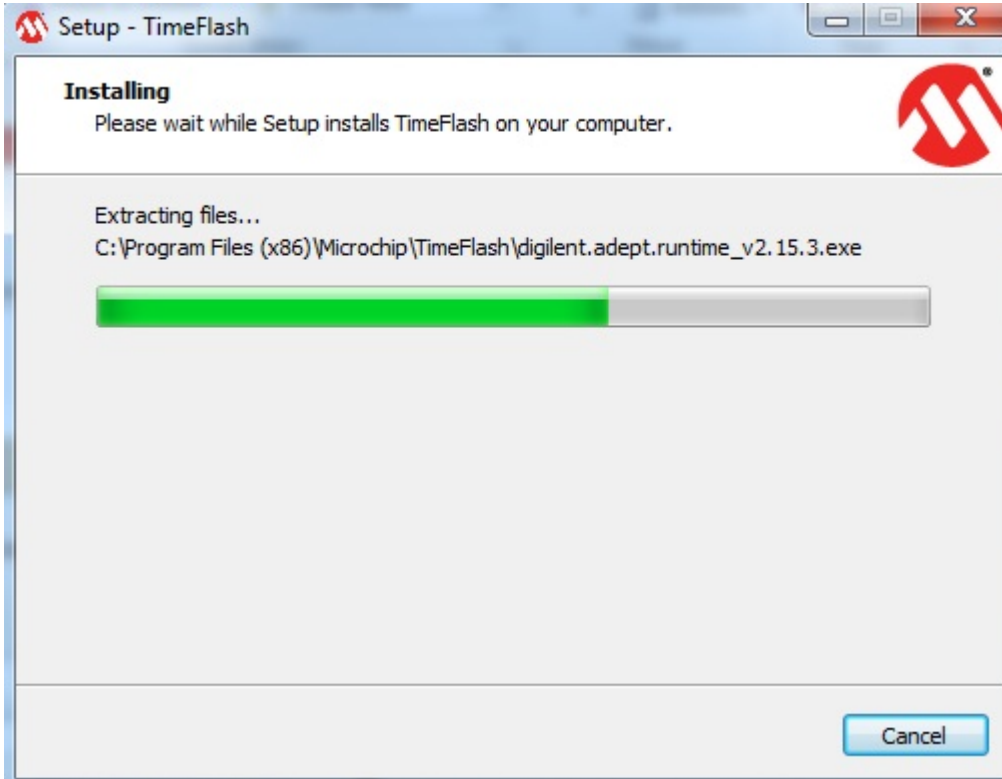
Figure 6: Installing TimeFlash 1.4
