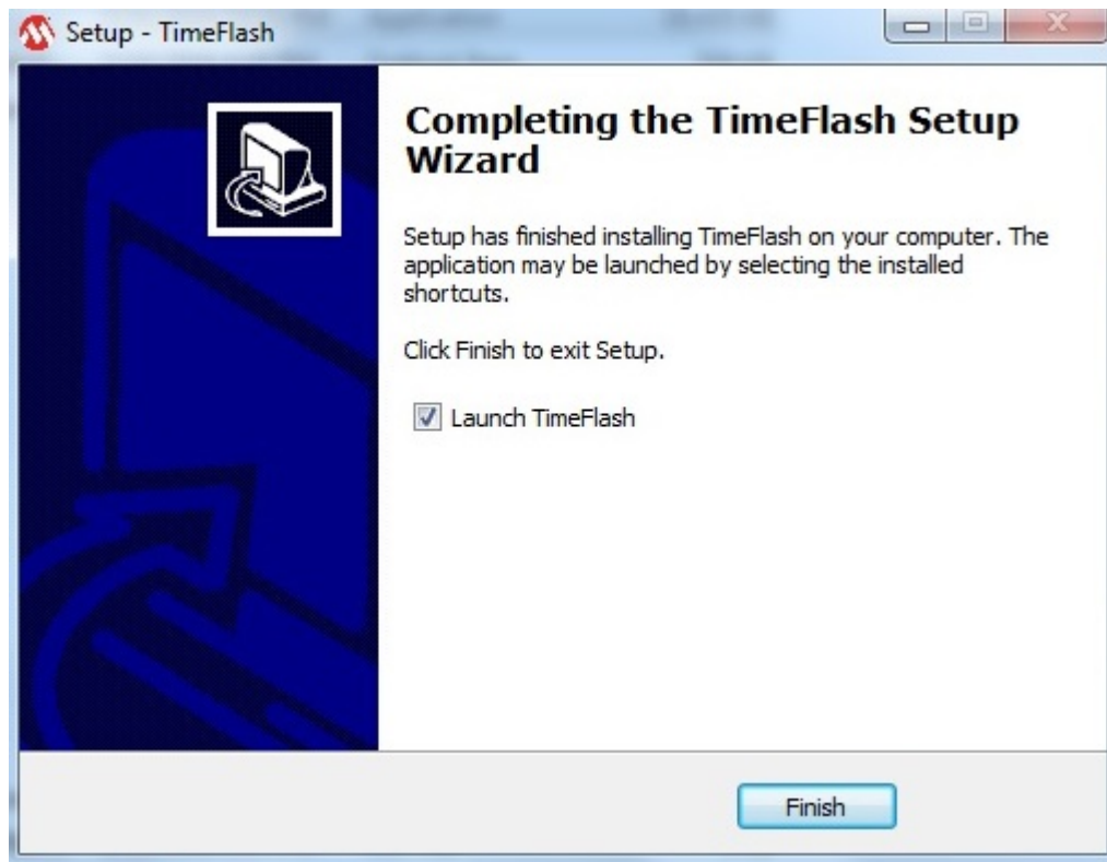
Figure 7: Installation Completed
