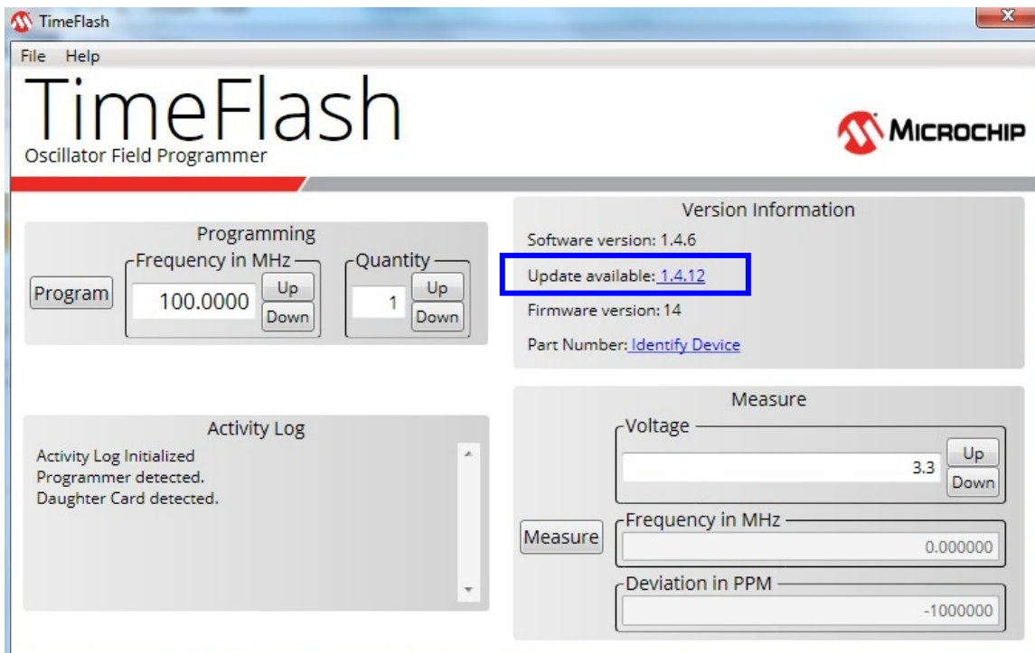
Figure 8: TimeFlash GUI
